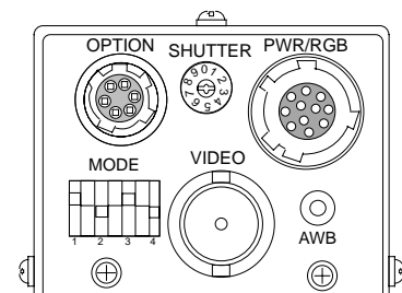
Rear panel
